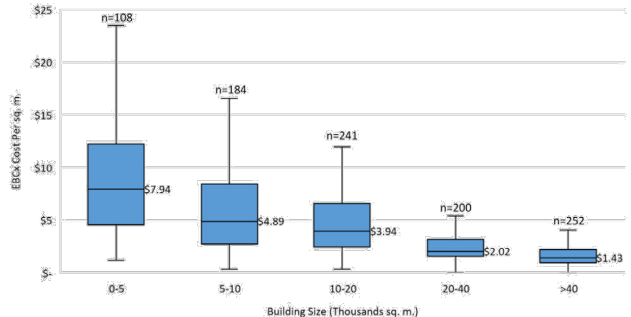
Fig. 4. EBCx project cost per square meter ($2017), by building size, with median values indicated (all data).
